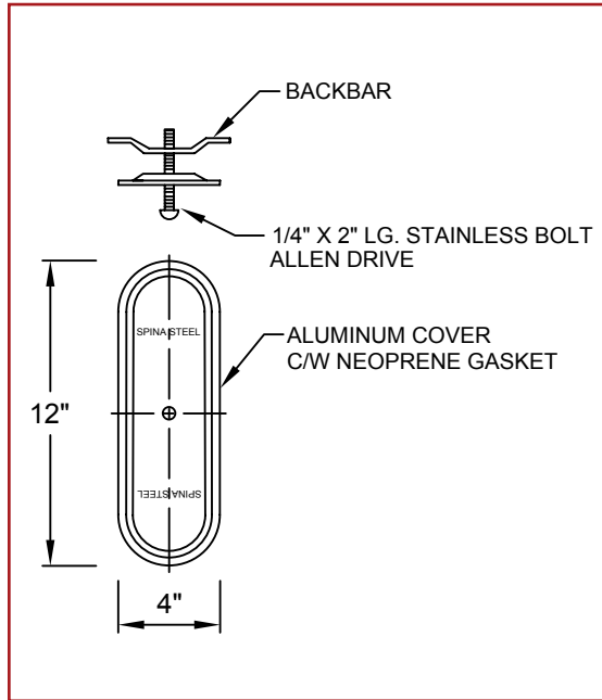
HANDHOLE COVER
