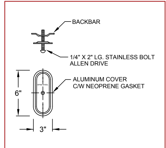
HANDHOLE COVER
